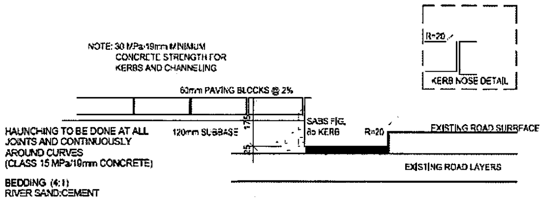
DETAIL OF SABS FIG 8b KERB FOR NEW CONSTRUCTION AT KEISER STREET
